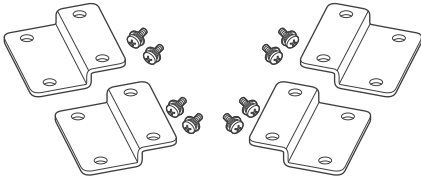
*Battery Fix Bracket (with 8 M4*12mm Fix Bolts)
